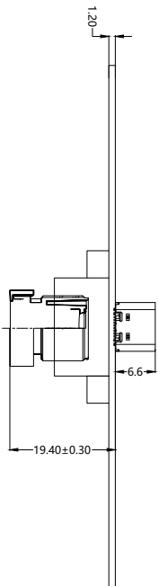
SIDE VIEW
